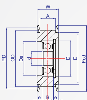
Single bearing
