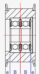
Two bearing
