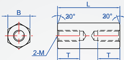
chamfer - 30°
